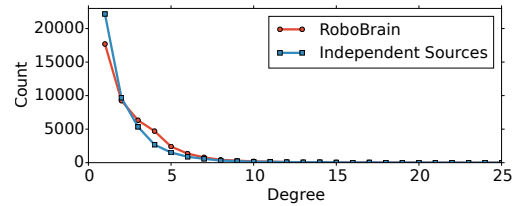
Fig. 9: Degree distribution of RoboBrain and the union of independent knowledge sources. For the case of independent sources, we only consider the edges between nodes from the same source. RoboBrain connects different projects successfully: number of nodes with degree 1 and 2 decrease and nodes with degree 3 and more increase.
